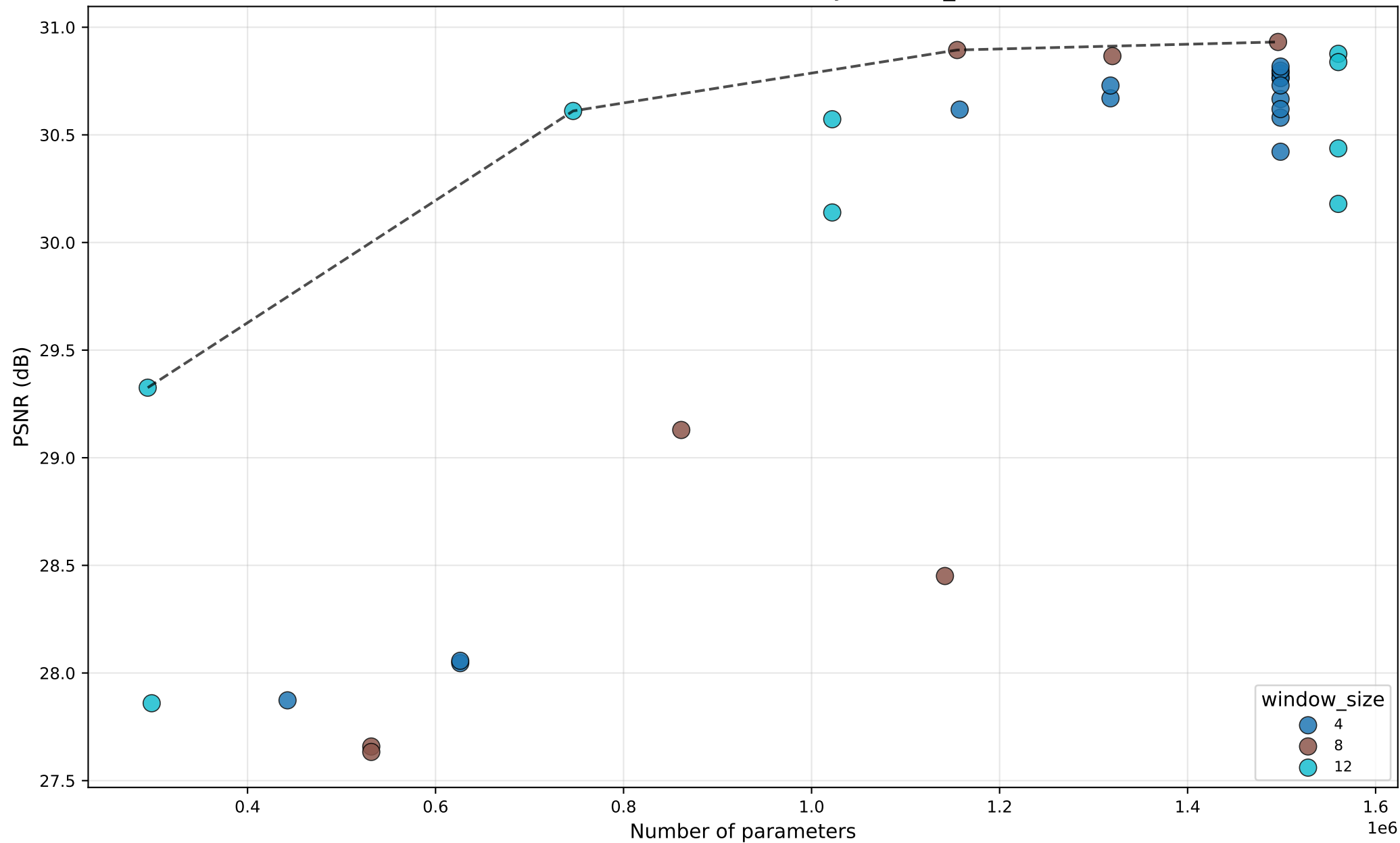
PSNR vs #Params — DAT — by window_size
